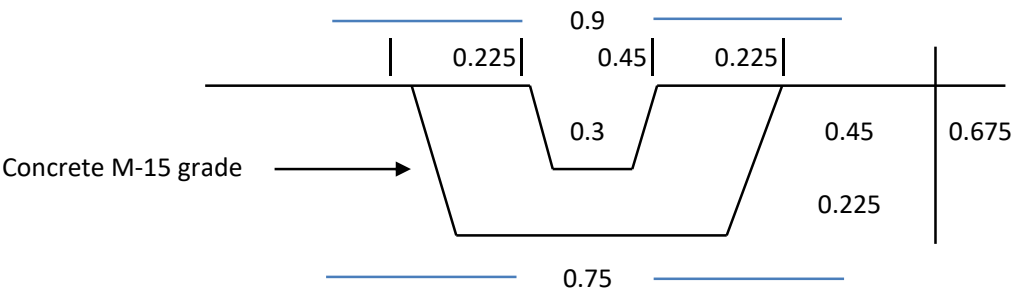
X-SECTION
